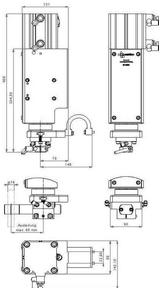
Picture: Dimension welding head SK-2020 without fixing/ mountings
